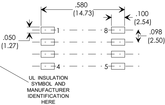
FIGURE 3: RECOMMENDED PCB LAYOUT DIMENSIONS IN INCHES (mm)
